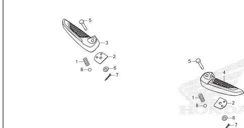
F-14-10 PILLION STEP (TIPE STREET)
